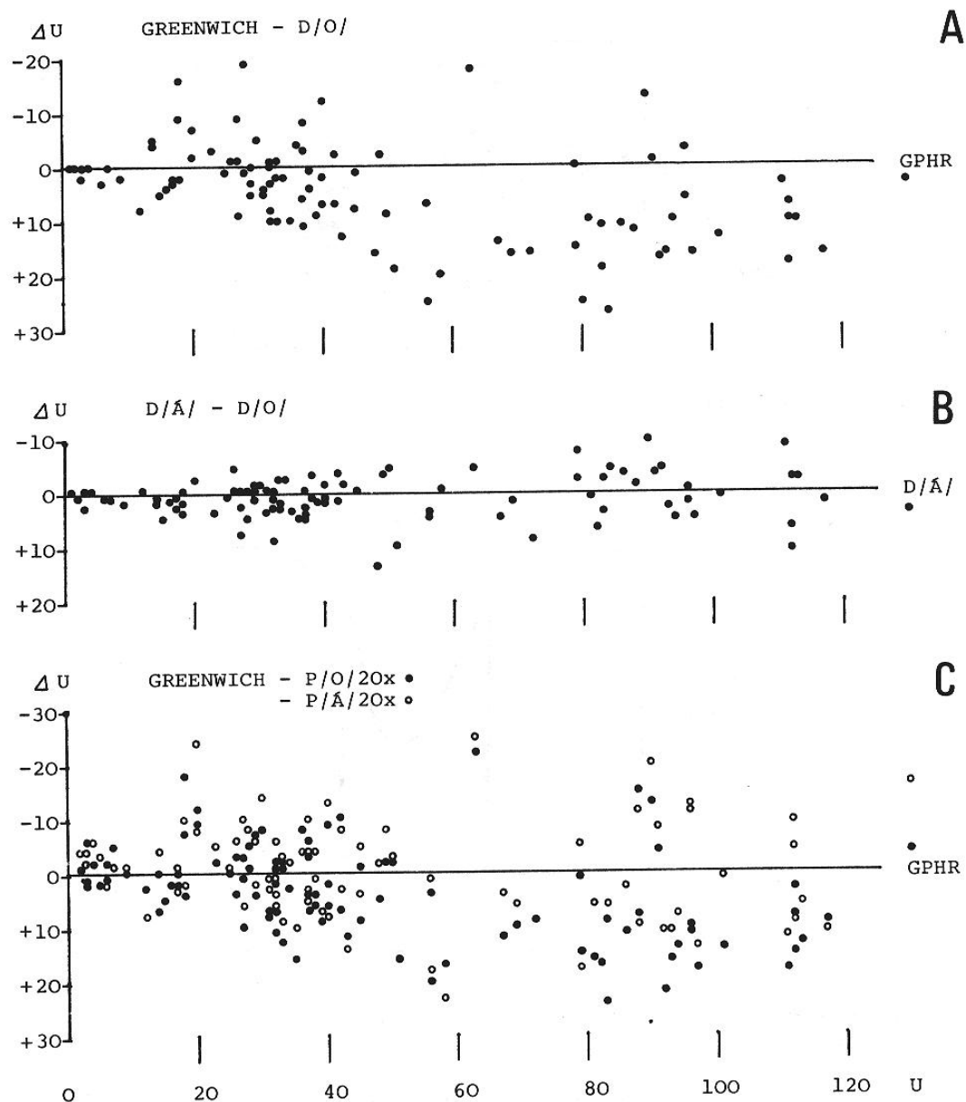
Fig.3.1 Various sets of differences in umbra area measurements ( \Delta U ) versus umbra area (U), in sample I.
