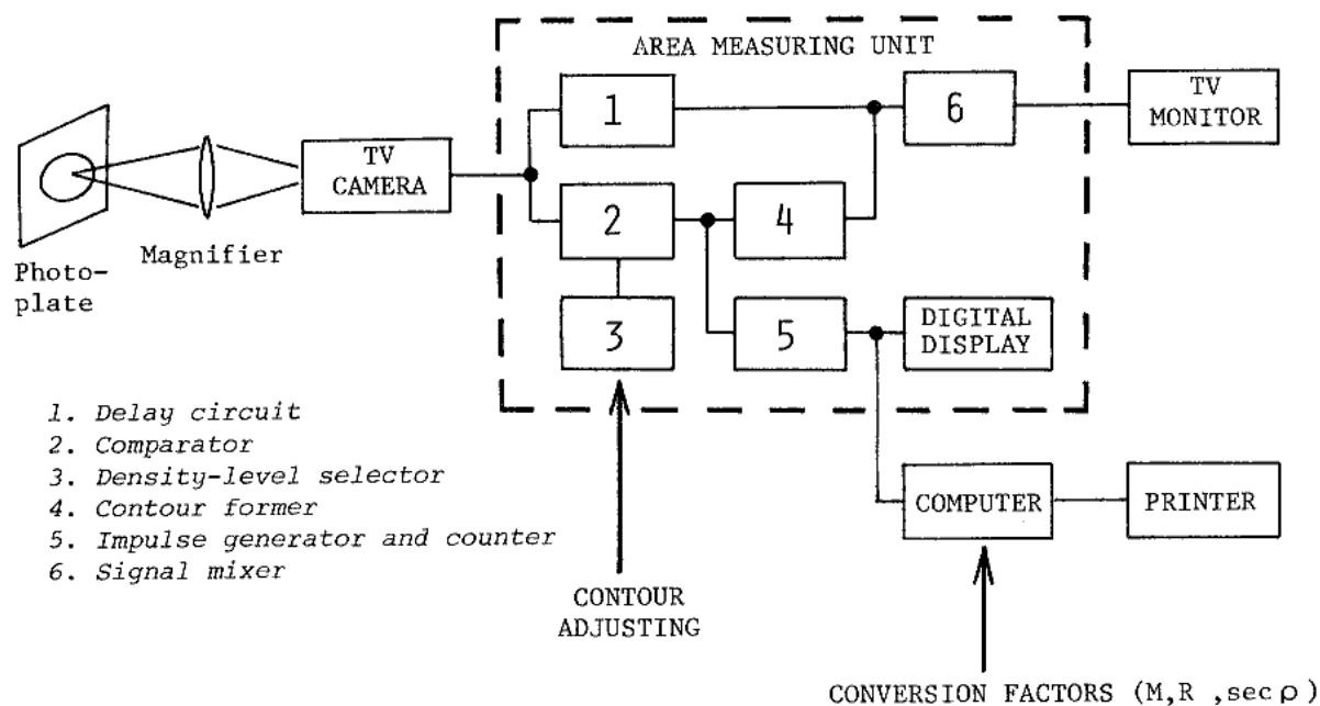
Fig.1 Schematic diagram of the Debrecen Area Measuring Instrument (DAREAL) (For the conversion factors M , R and \sec \rho see the text.)
